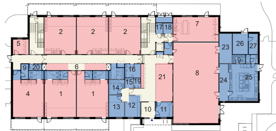
Proposed Ground Floor Plan NTS
